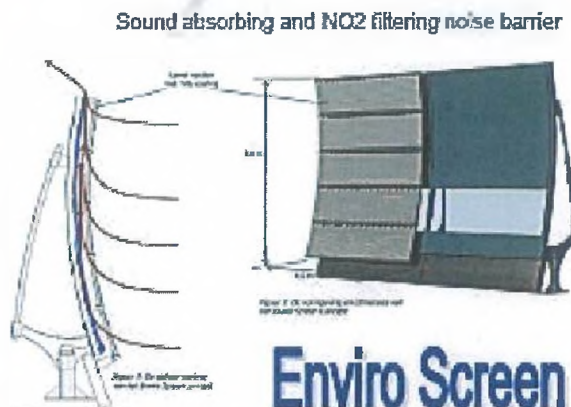
Sound absorbing noise barrier
